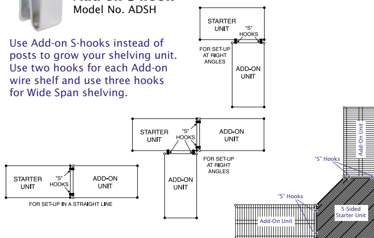
Add-on S-hook Model No. ADSH
